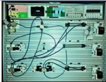
Electro- Pneumatic Trainer Kit (Rs.1,47,000/-)
